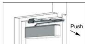
Parallel Arm Installation Closer Installed in "Push" Side of the Door
