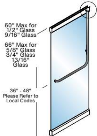
ITEM NO. DHP100 Dummy Handles
