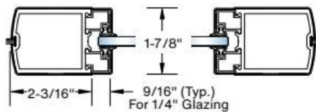
Single Door
