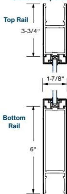
Standard Top and Bottom Rails
