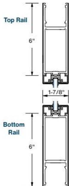
Standard Top and Bottom Rails
