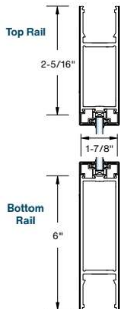
Standard Top and Bottom Rails
