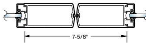
Meeting Stiles for Pair of Doors
