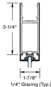
Top Rail
