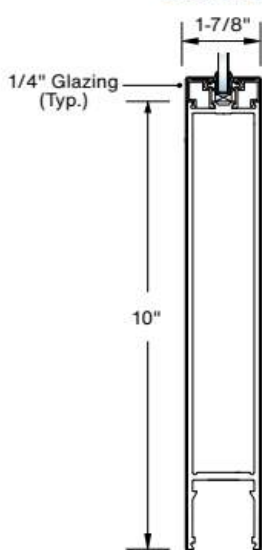
Optional: 10" A.D.A. Bottom Rail
