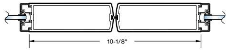
Meeting Stiles for Pair of Doors
