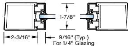
Standard Top and Bottom Rails
