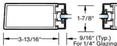
Standard Top and Bottom Rails
