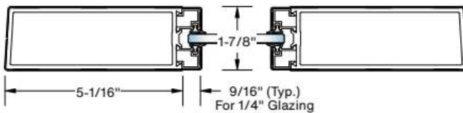
Standard Top and Bottom Rails
