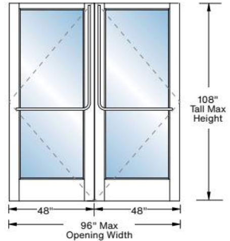
Meeting Stiles for Pair of Doors
