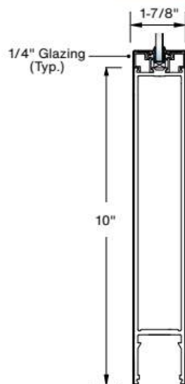
Optional: 10" A.D.A. Bottom Rail
