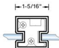
Partition Center Post
