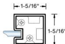
Partition End Post
