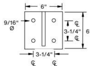
Mounting Plate Detail
