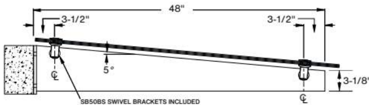
AWBS48 48" Glass Awning Bracket
