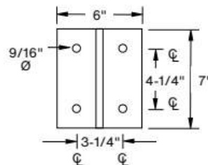
AWBR36 Mounting Plate Detail
