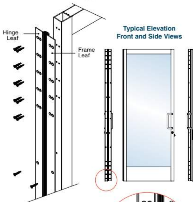
Typical Continuous Hinge Door Layout
