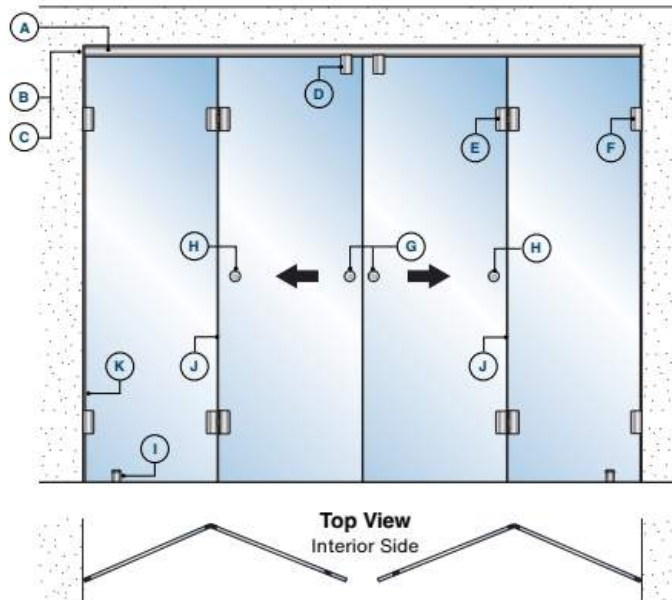
FHC ANDREA SERIES FRAMELESS BI-FOLDING SLIDING DOOR SYSTEM COMPONENTS
