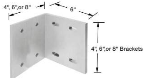
FHC END MOUNTING SUNSHADE BRACKETS
