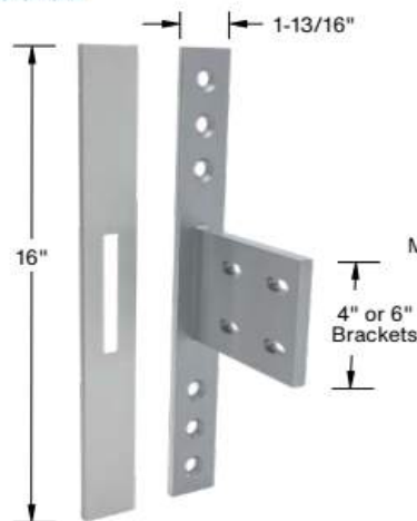
FHC STOREFRONT SUNSHADE BRACKET
