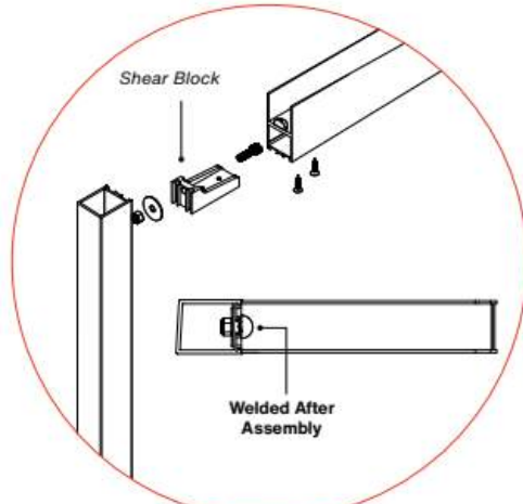
TYPICAL TOP SETTING BLOCK DETAIL
