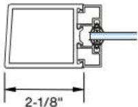
200 SERIES NARROW STILE
