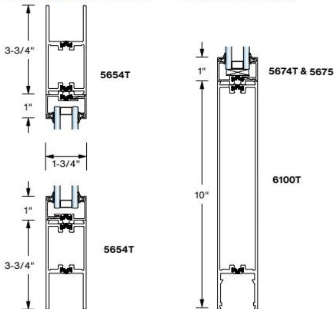
Standard Top and Bottom Rails
