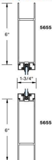
Standard Top and Bottom Rails
