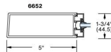
Standard Top and Bottom Rails
