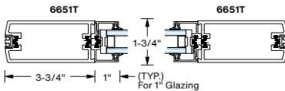
Single Door
