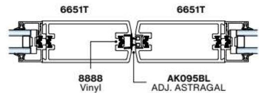
Meeting Stiles for Pair of Doors
