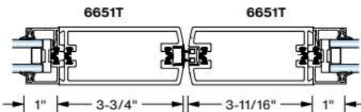
Meeting Stiles for Pair of Doors
