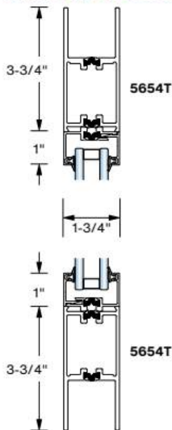
Standard Top and Bottom Rails
