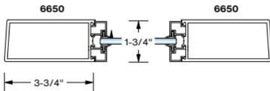
Standard Top and Bottom Rails
