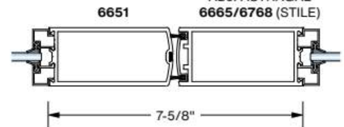
Meeting Stiles for Pair of Doors
