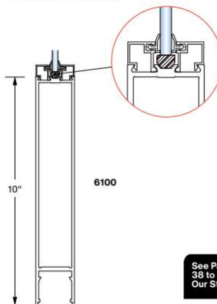
10" A.D.A. Bottom Rail
